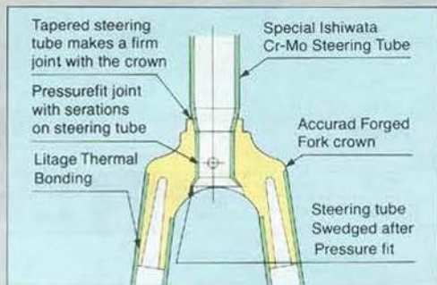
Litage Dual Bonding Process
