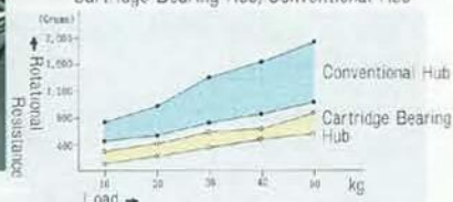
ROTATIONAL RESISTANCE UNDER LOAD Cartridge Bearing Hub/Conventional Hub
